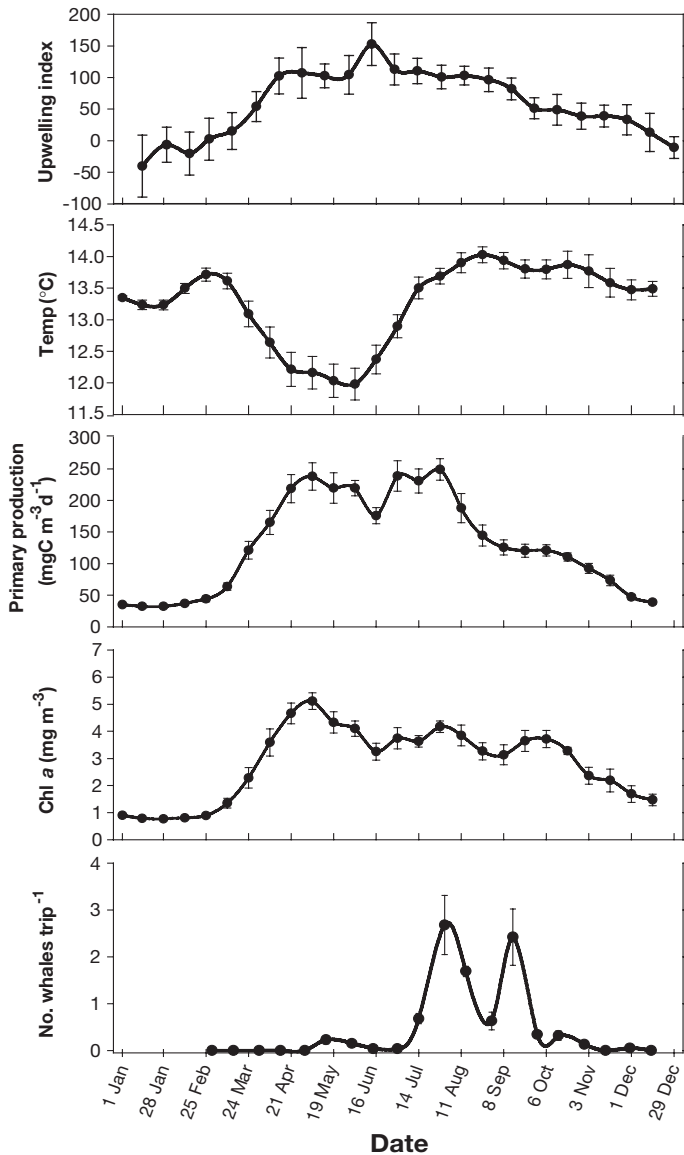
Fig. 3. Oceanographic climatology (mean ± SD) for Monterey Bay, California between 1992 and 1996, showing from top to bottom: Pacific Fisheries Environmental Laboratories/NOAA upwelling indices, sea-surface temperature, primary production at 100% light levels, integrated chlorophyll a , and number of whales Baleanoptera musculus per trip in opportunistic whale-watch surveys
